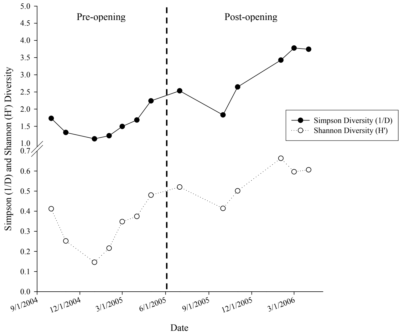
Figure 13. Indices of species diversity for nekton by sampling date with all locations combined. The solid line represents the reciprocal of the Simpson index ( 1/D ) and the dashed line represents the Shannon index ( H' ). The dashed vertical line divides pre-opening (October 2004 – May 2005) from post-opening (July 2005–April 2006).
