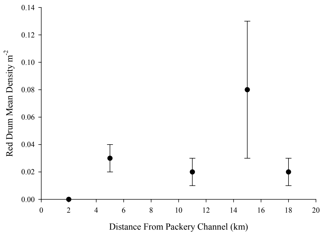
Figure 5. Relationship between mean red drum density ( \text{m}^{-2} \pm \text{SE} ) and distance from Packery Channel (km) in fall 2005 post-opening analyzed with simple linear regression. Regression model: \text{density} = 0.001 (\text{distance}) + 0.002 ; N = 5 , R^2 = 0.369 , P = 0.277 .
