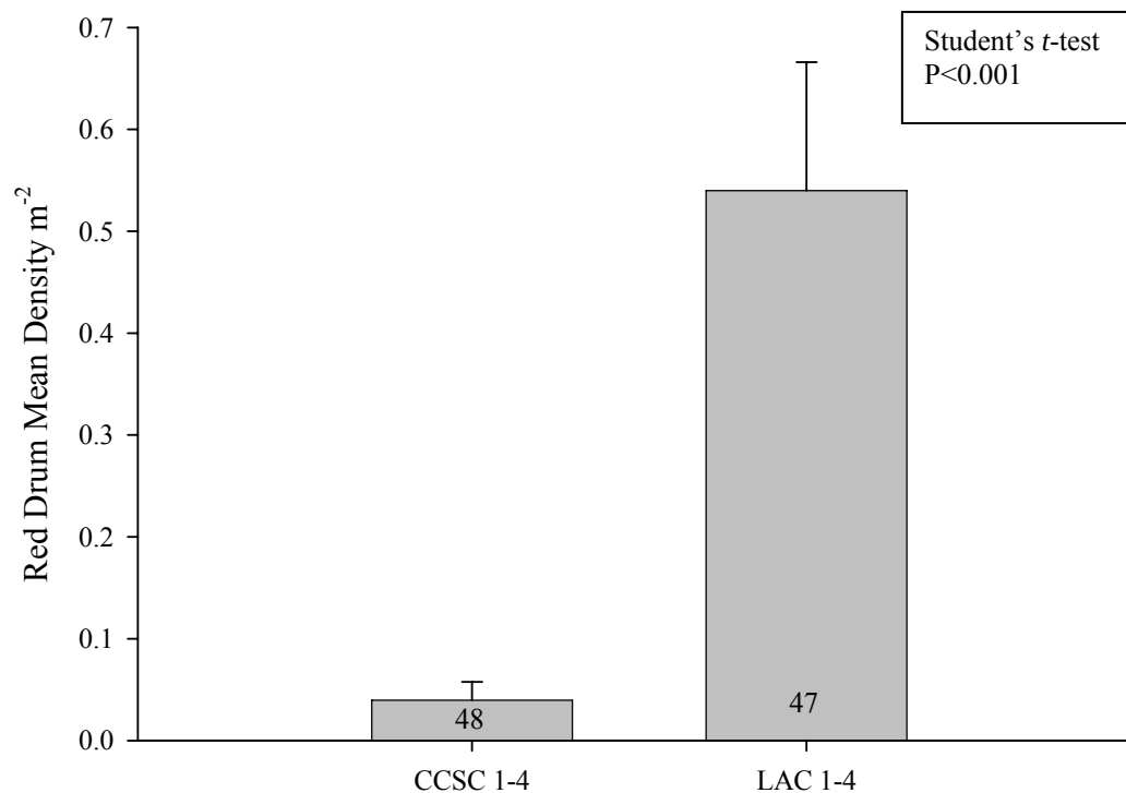
Figure 23. Mean red drum densities ( \text{m}^{-2} \pm \text{SE} ) in the Corpus Christi Ship Channel (CCSC) and Lydia Ann Channel (LAC). Densities were combined from all sampling events and sites within the CCSC and LAC. Sites 1-4 were located along each of the channels and were on bare bottom in the CCSC and in seagrass in the LAC. The number of samples taken in each channel is indicated at the bottom of each bar. Densities of red drum in each channel were analyzed using a Student's t -test.
