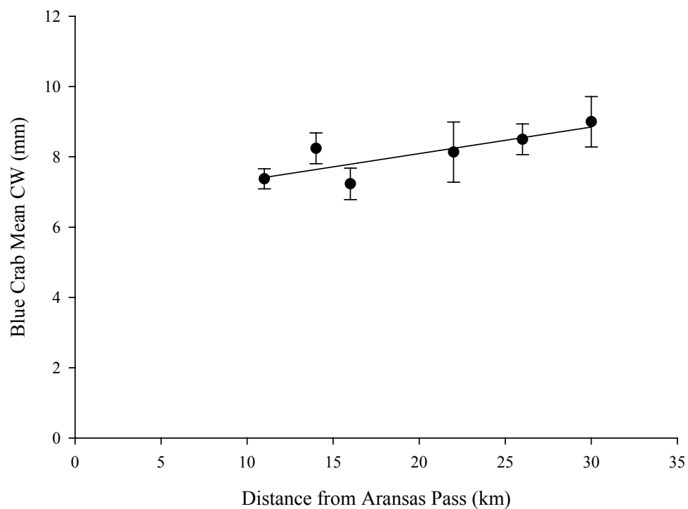
Figure 14. Blue crab mean CW ( \pm SE) at varying distances from Aransas Pass post-opening of Packery Channel. The relationship between mean CW and distance from Aransas Pass was analyzed using a simple linear regression. Regression model: CW = 0.00359 (\text{distance}) + 0.887 ; N = 6 , R^2 = 0.664 , P = 0.048 .
