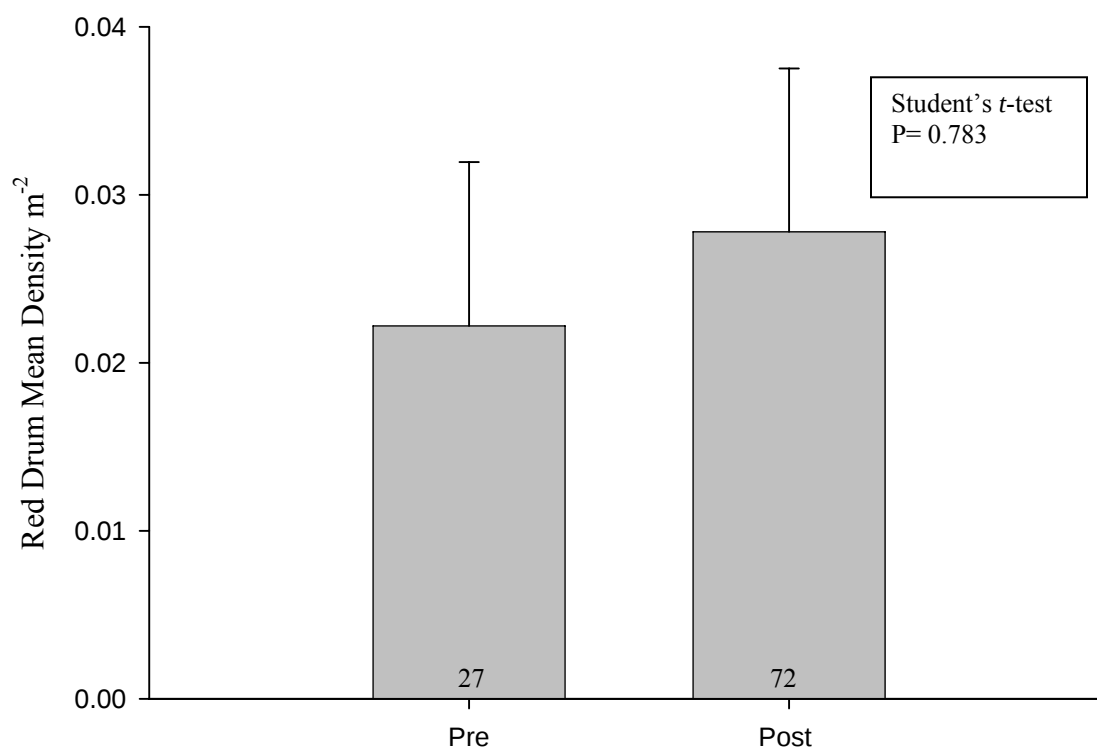
Figure 8. Mean red drum densities ( \text{m}^{-2} \pm \text{SE} ) at sites surrounding Packery Channel pre- and post-opening. Densities were analyzed using a Student's t -test. The number of samples for pre- and post-opening is indicated at the bottom of the bars.
